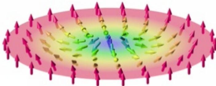
Figure 7: A field configuration with winding number Q = 1 . Notice that no continuous change in the spin directions can transform this to a configuration where all spins point upwards. (Figure by Karin Everschor-Sitte and Matthias Sitte).
